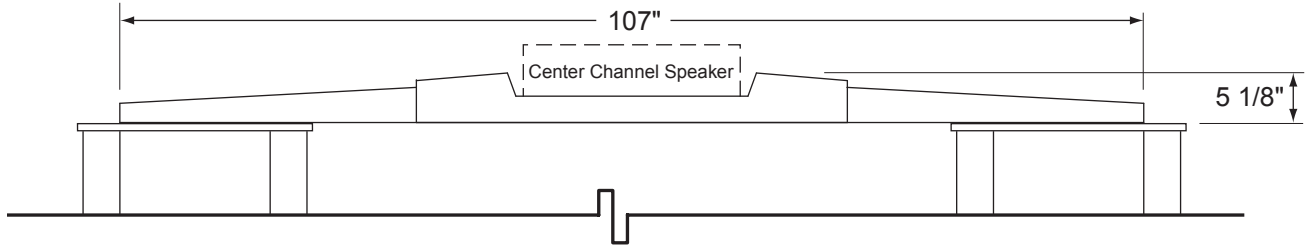
FRONT VIEW (Video Bridge for Center Channel Speaker)
